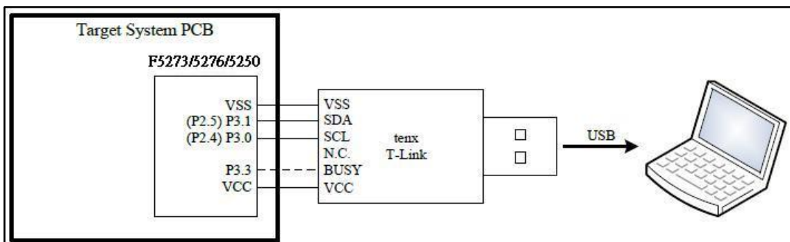
Figure 2-1. T-Link-EV5273/5276/5250 Board
