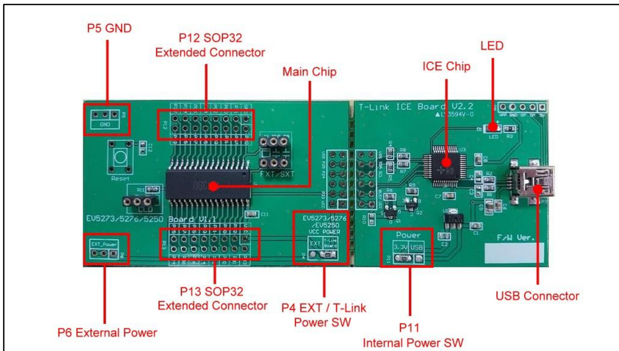
Figure 2-1. T-Link-EV5273/5276/5250 Board
