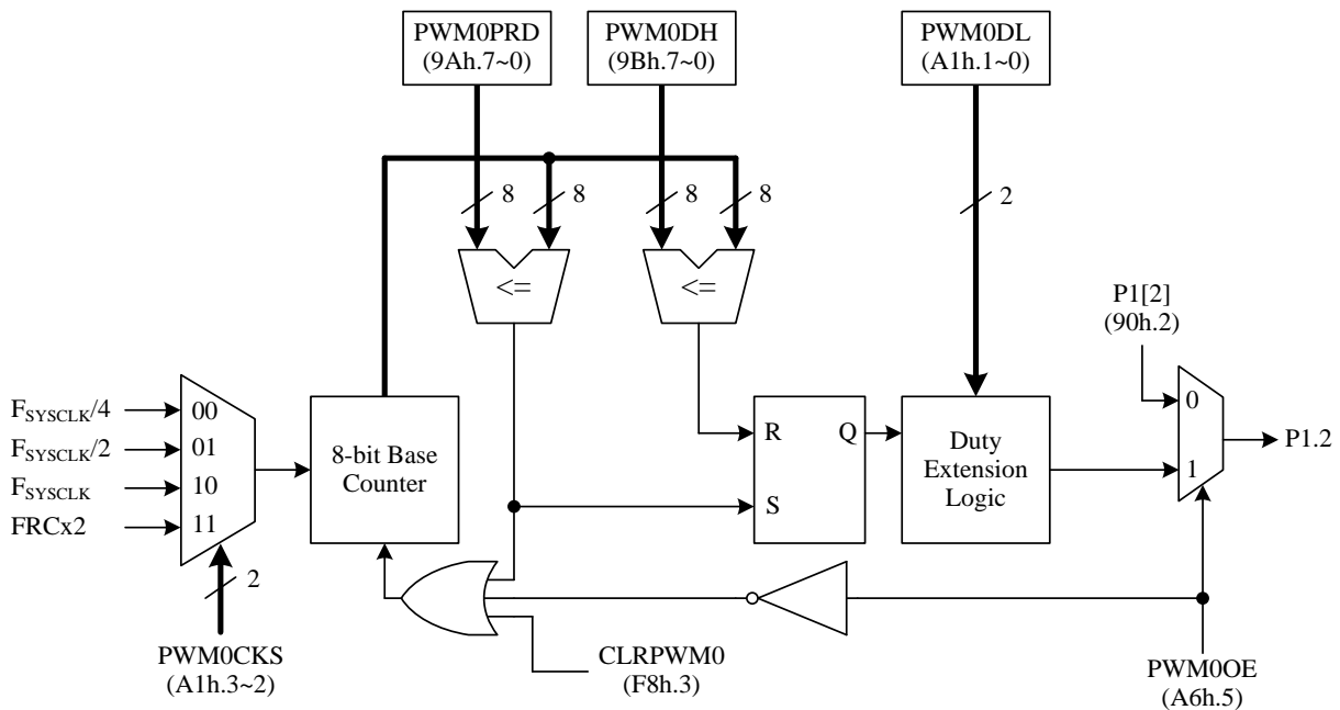
PWM Structure
