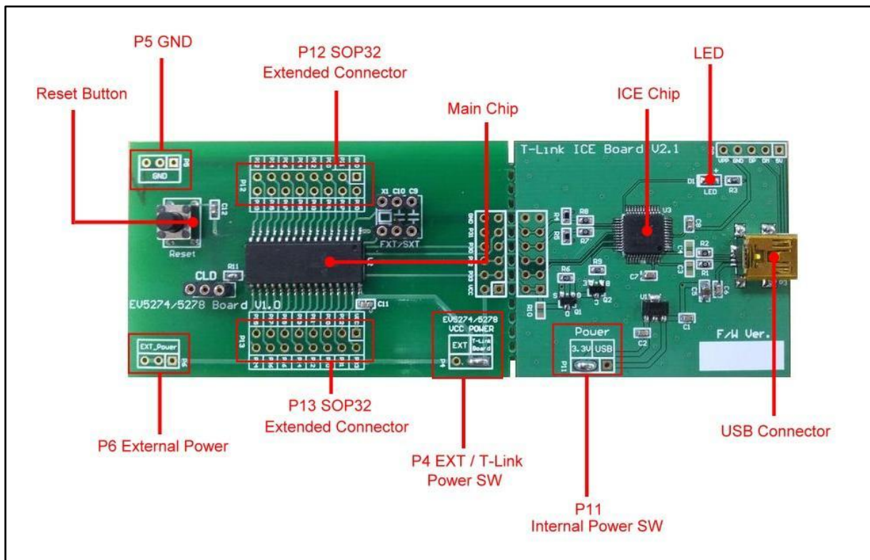
Figure 2-1. T-Link-EV5274/5278 Board
