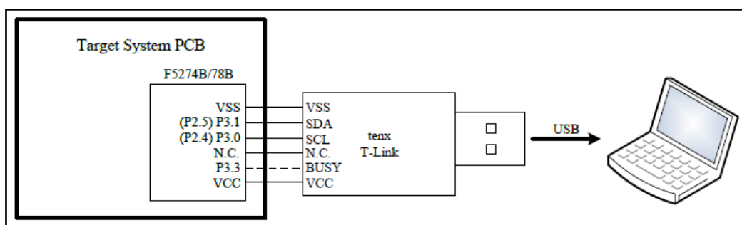
Figure 2-1. T-Link-EV5274/5278 Board
