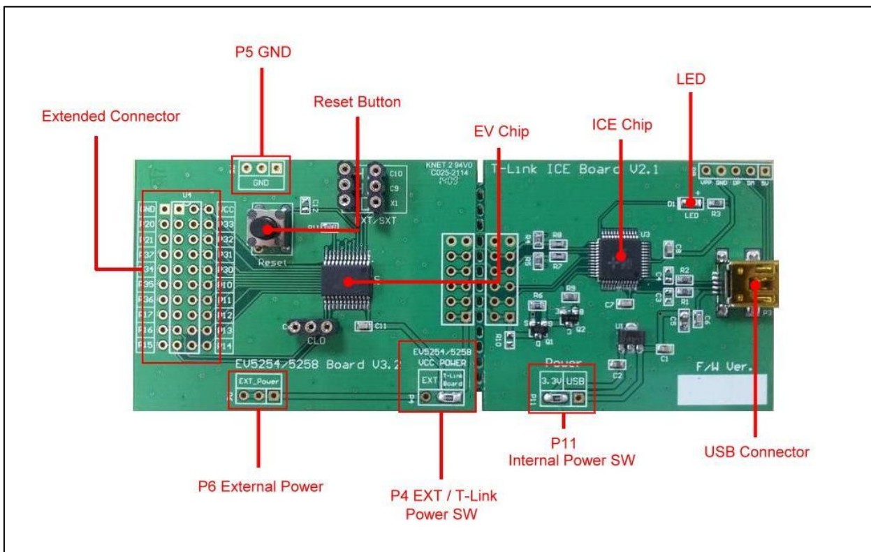
Figure 2-1. T-Link- EV5254/5258 Board
