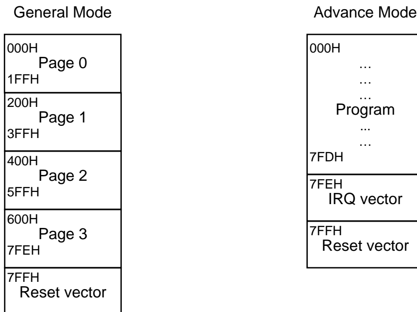
Figure 5-1 The ROM Organization
