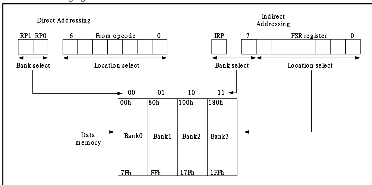
BANK 0/1/2/3 direct/indirect addressing
