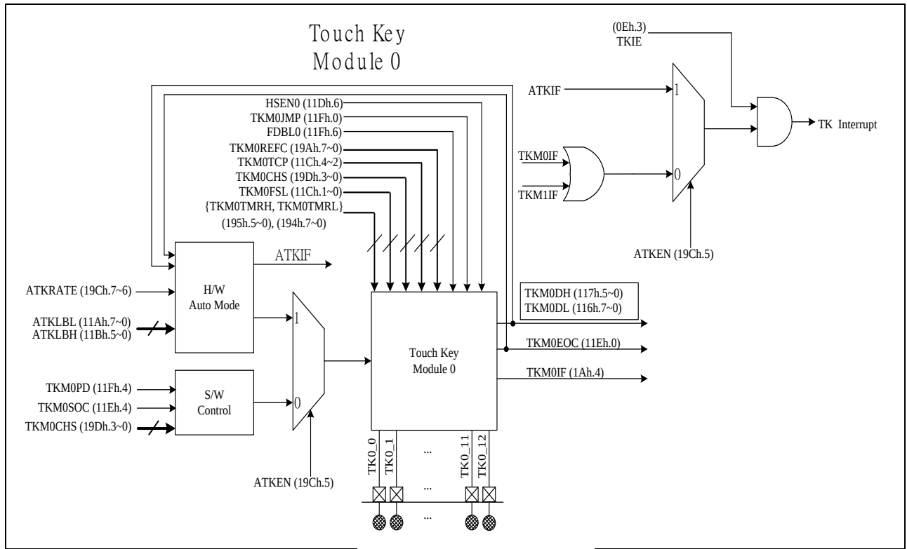
Touch module 0/ATK structure
