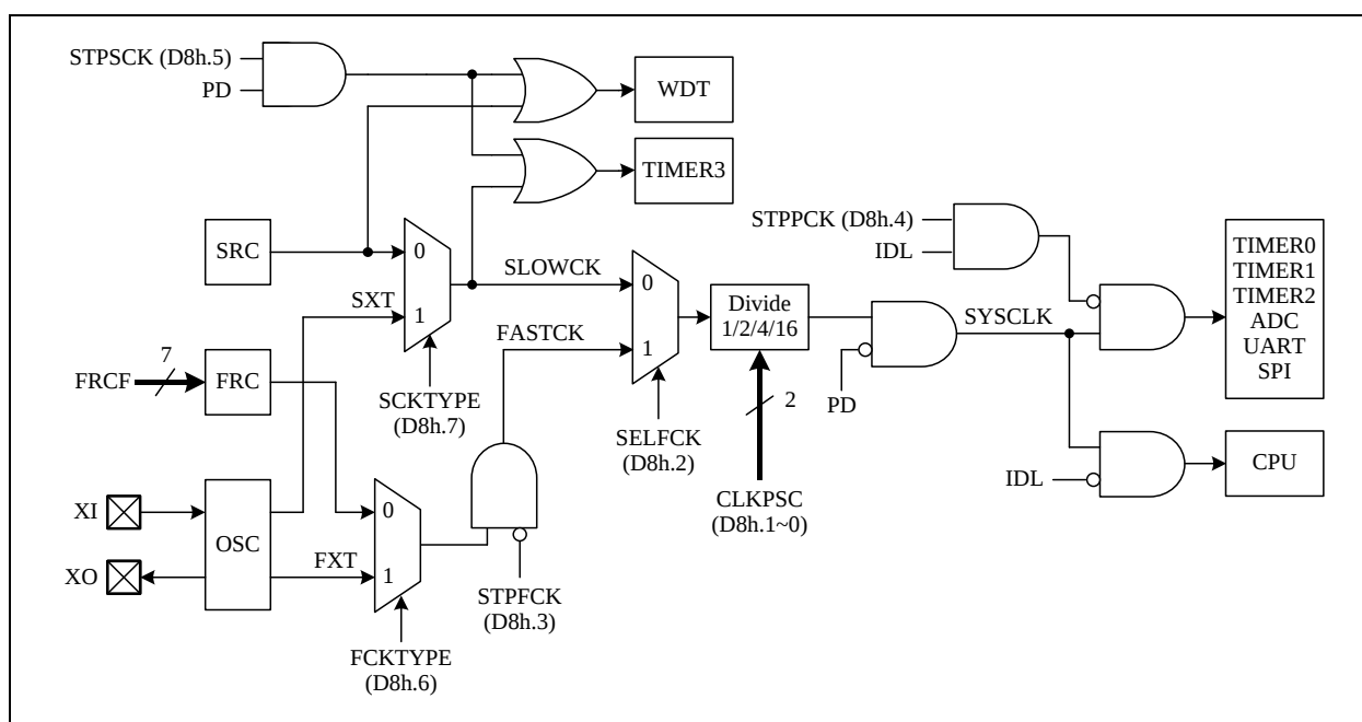
Clock Structure
