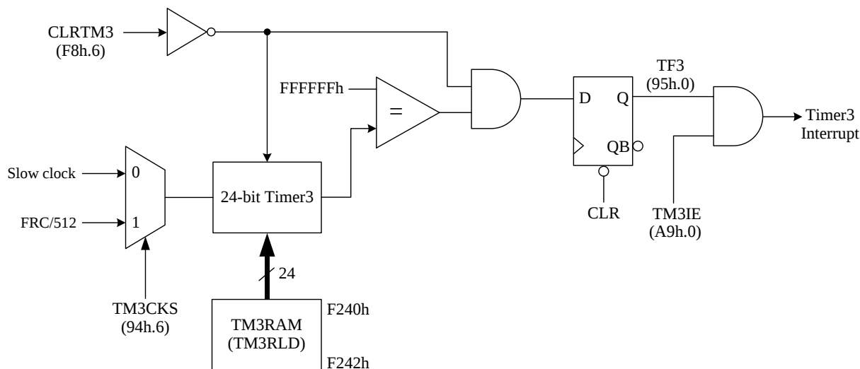
Timer3 Structure
