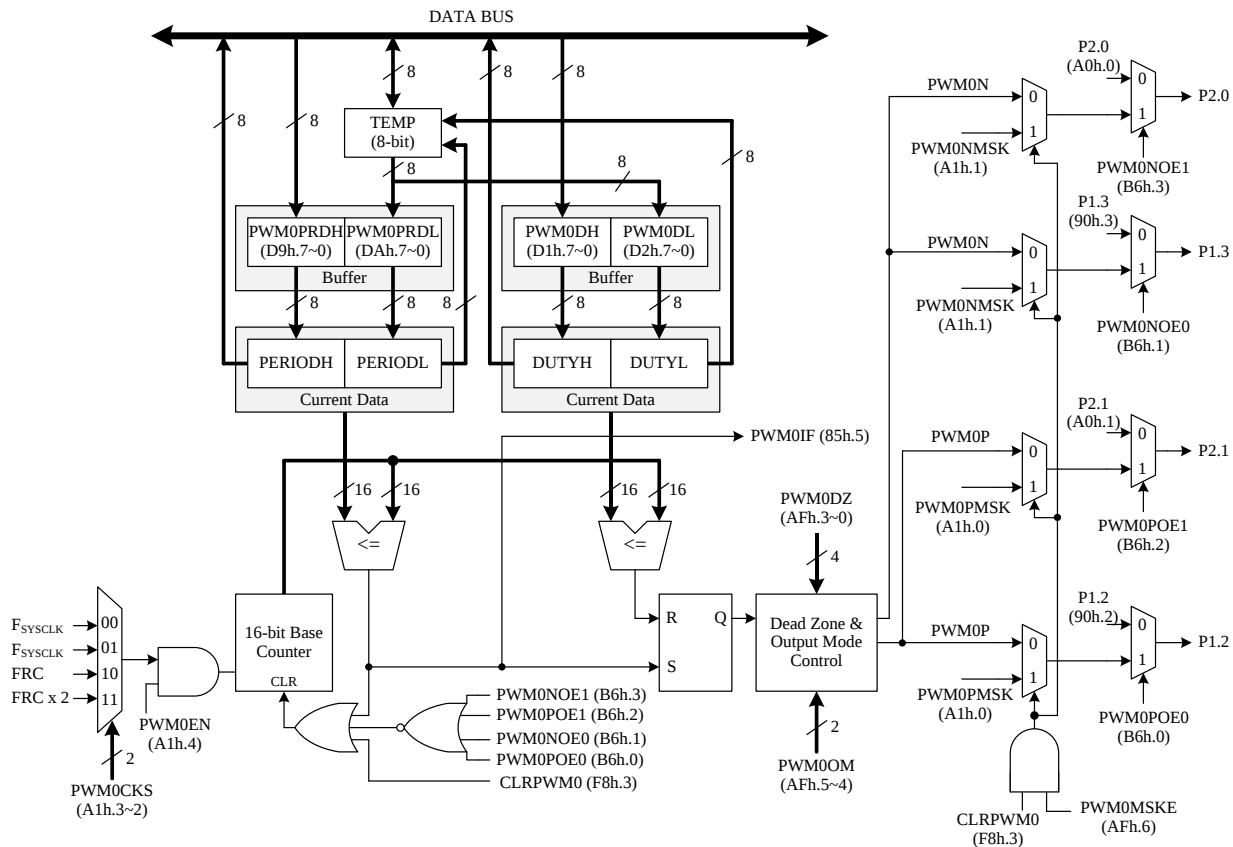
PWM0 Structure
