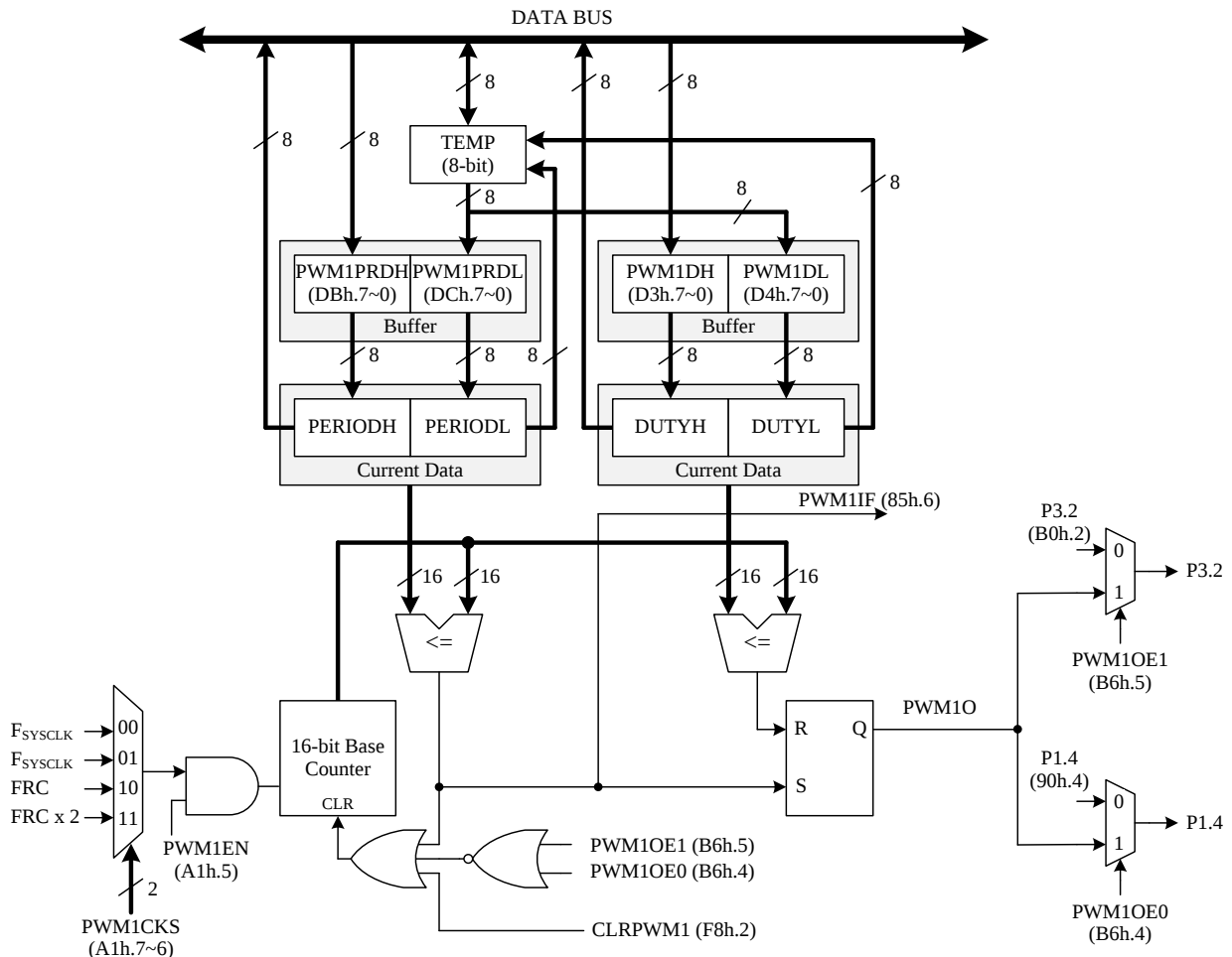
PWM1~6 Structure
