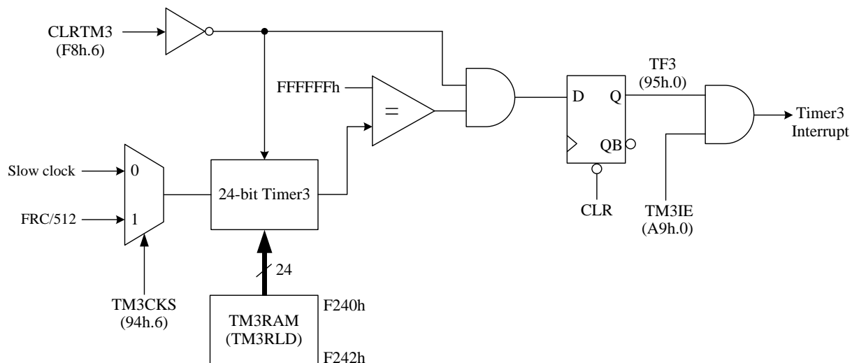
Timer3 Structure
