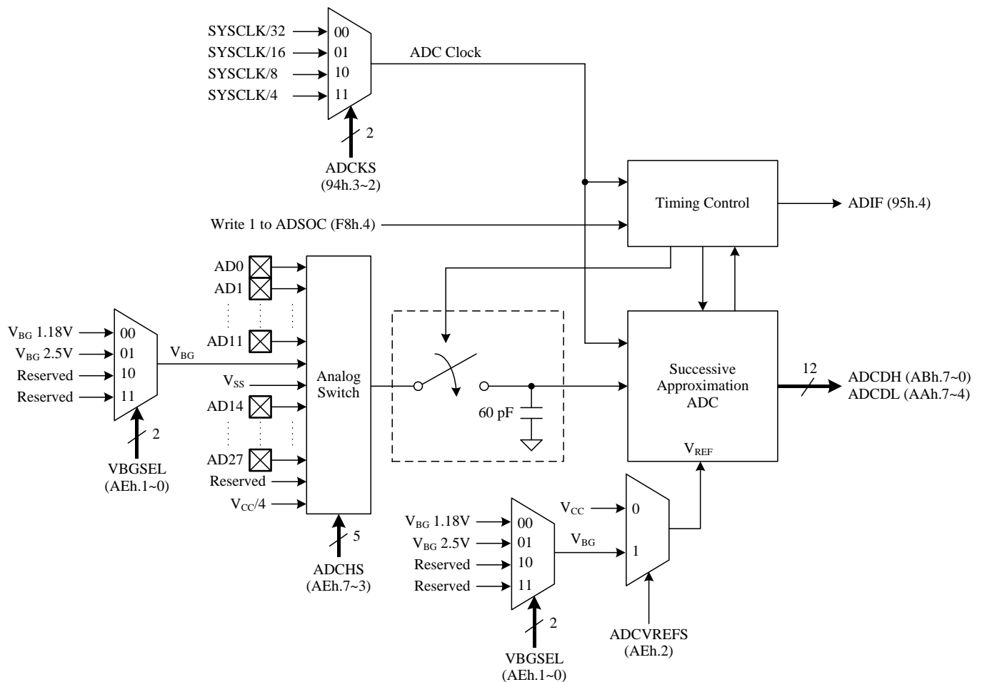
ADC Structure
