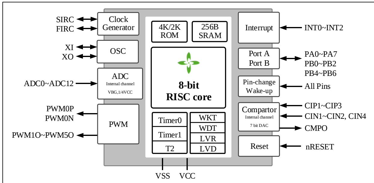
TM56M1522/22C/22L/21H/21C Block Diagram
