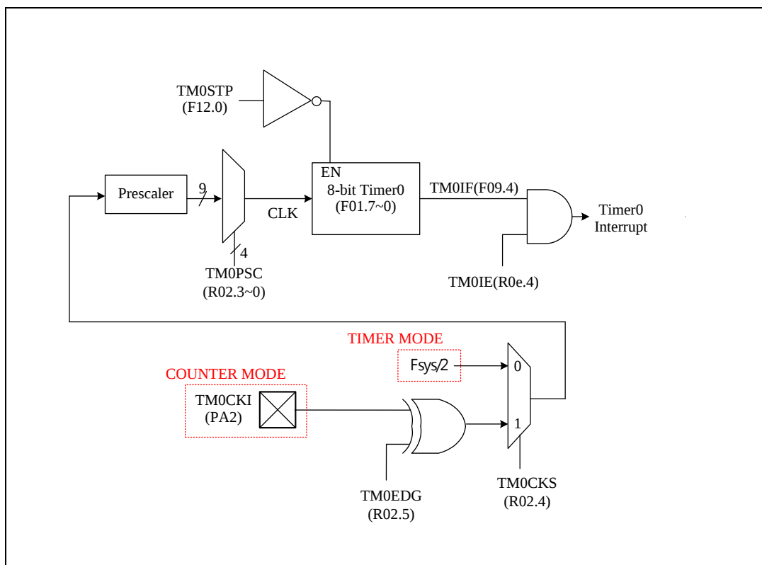
Timer0 Block Diagram
