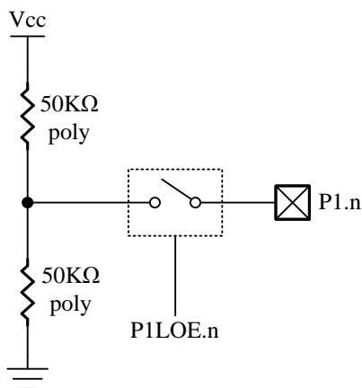
LCD COM0~3 Circuit
